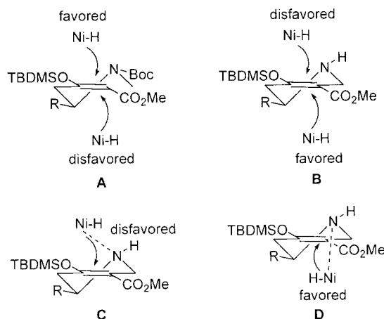
Figure 2. Stereochemistry analysis for hydrogenation of 6 (A) and 13 (B, C, and D).
